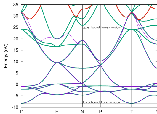
Fig. 1: Comparison of the explicit (green lines) and Wannier-interpolated (magenta lines) DFT band structure for iron (spin-up). The Wannier functions are constructed with ORBITALS 1 * (s, p, d) , MAXIMIZE , and FROZEN . The lower bound of the outer energy window is set at the lowest valence band (band index 1), and the upper bound is set automatically by Spex (wildcard “*”). In this case, it is set to the 12th band, here marked in red. The lower and upper bounds of the inner frozen energy window for disentanglement are guessed by Spex and shown in the figure as well.
